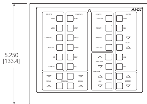
TXC32+ (Front, with engraved overlay)
