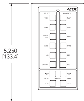
TXC16+ (Front, with engraved overlay)
